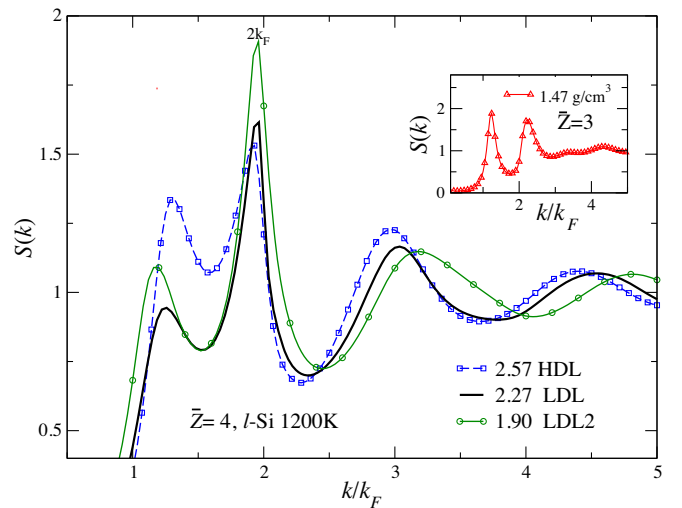
FIG. 3. The structure factor S(k) of LPT2.5 and LPT2 at 1200 K. The main split-off-peak registers at 2k_F as required by the Fermi liquid picture (this holds for LPT3 also, though not displayed). The x axis is k/k_F with k_F appropriate to \bar{Z} = 4 . The inset for S(k) at 1.47 \text{ g/cm}^3 , \bar{Z} = 3 , is beyond the IDT, and shows no 2k_F splitting.
