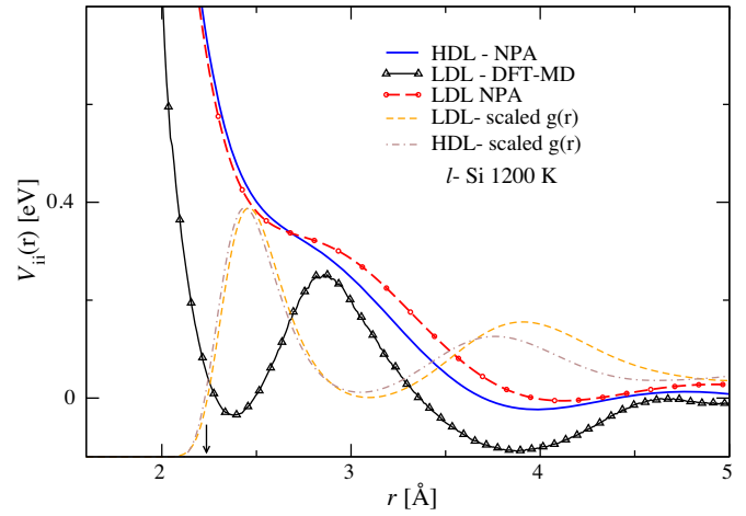
FIG. 5. The ion-ion potentials of the HDL and LDL are shown against their PDFs (scaled to match the potentials). The arrow at r_b marks the Si-Si bond length. The first shell of ions sits on a repulsive ledge stabilized by the electron cohesive energy, while the second shell is in a Friedel-oscillation minimum (FOM). The HDL \rightarrow LDL involves a cooperative movement of ions to the second shell as seen in the enhanced LDL g(r) in the FOM region. This picture holds also for the LPT2 and LPT3 (see [33]). The DFT-SCAN potential accommodates the first shell at its true minimum.
