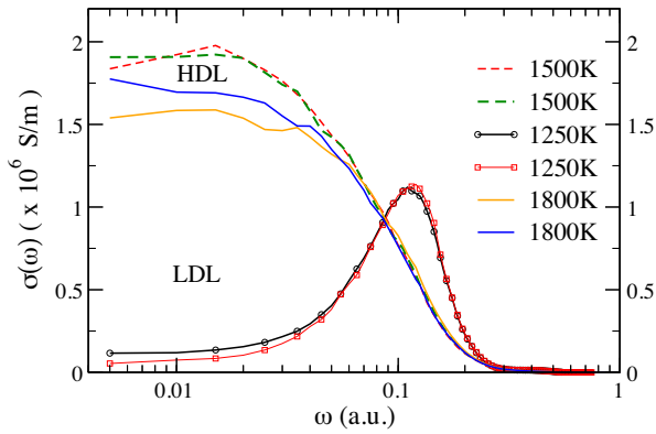
FIG. 6. \sigma(\omega) from DFT-MG-KG. for and HDL and LDL Si at LPT2.5. The LDL has a striking finite \sigma(\omega) , but the static \sigma indicates a nearly nonmetallic LDL.
