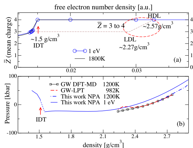
FIG. 1. (a) The Si charge \bar{Z} versus the free electron density n_f . At low density, a drop in \bar{Z} may cause an ionization driven transition (IDT). The ellipse indicates the HDL-LDL LPT. (b) The HDL branch of the Ganesh-Widom (GW) pressure [16] and the NPA at 1200 K agree. The pressure at 1 eV (11 604 K) is discontinuous at the IDT.
