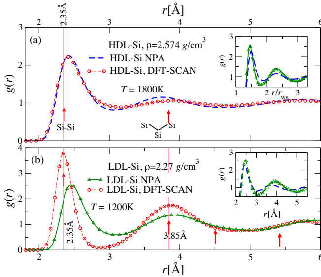
FIG. 4. g(r) of (a) HDL ( 2.57 \text{ g/cm}^3 ) Si from NPA and from DFT-SCAN at 1800 K, (b) LDL ( \sim 2.27 \text{ g/cm}^3 ) Si from NPA and DFT-SCAN. The Si-Si bond length ( 2.35 \text{ \AA} ) is indicated. The NPA-HNC fails to capture the increased g(r) at 2.35 \text{ \AA} and remain locked in an HDL-like structure. Insets: the NPA g(r) , for HDL-Si and LDL-Si versus r/r_{\text{ws}} , and with r in \text{\AA} . The HDL r_{\text{ws}} \simeq 3 \text{ a.u.}
