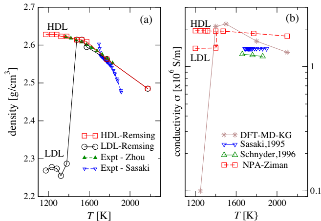
FIG. 7. (a) The density \bar{\rho} versus T from DFT-SCAN [20] near LPT2.5 is compared with available experimental densities. (b) The static conductivity \sigma from NPA-Ziman, DFT-KG and from experiments [51,52].
